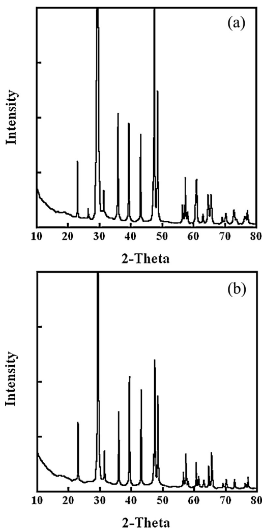
Fig. 2. XRD diffraction patterns of commercial calcium carbonate (a) and eggshell powder (b).
