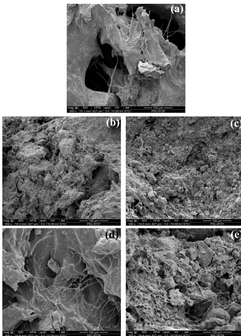
Fig. 6. SEM micrographs of TPS (a), TPS/CC composites with: 10 wt.% (b) and 30 wt.% (c) of commercial calcium carbonate and TPS/EP composites with: 10 wt.% (d) and 30 wt.% (e) of eggshell powder after the soil burial test for 15 days.
