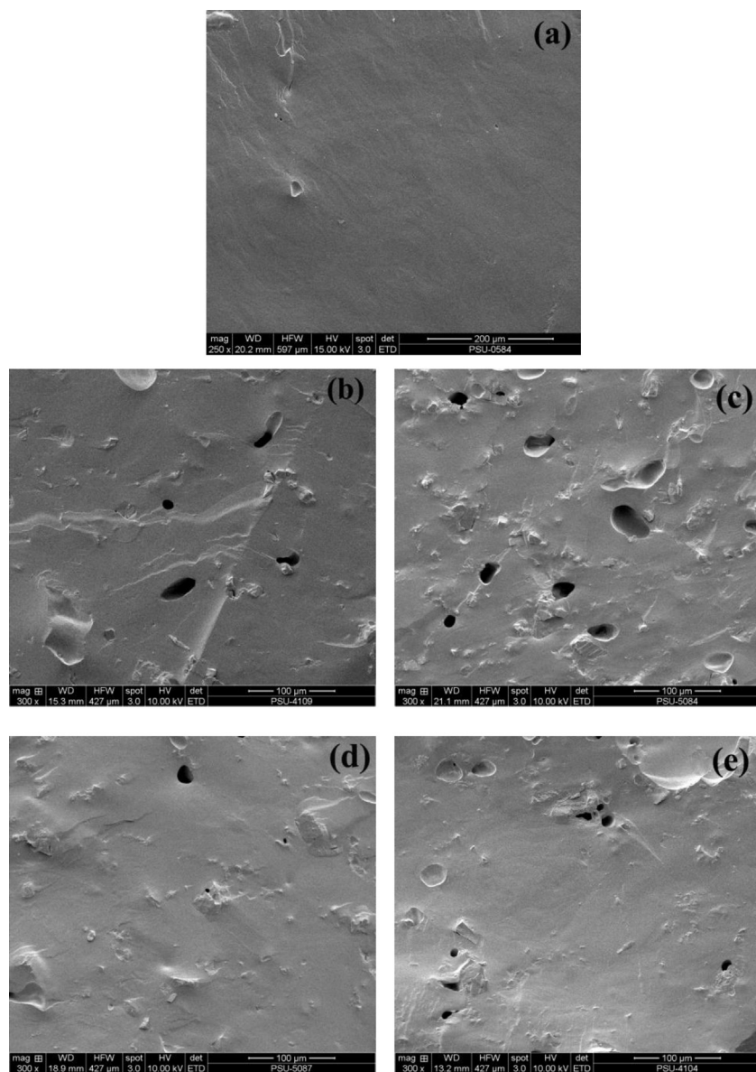
Fig. 3. SEM micrographs of TPS (a), TPS/CC composites with: 10 wt.%(b) and 30 wt.%(c) of commercial calcium carbonate and TPS/EP composites with: 10 wt.%(d) and 30 wt.%(e) of eggshell powder.
