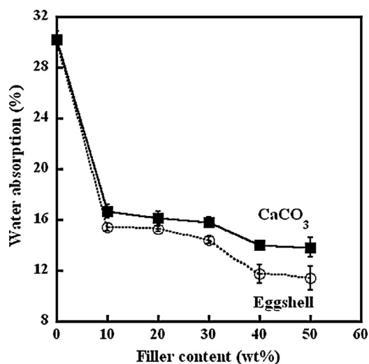
Fig. 4. Water absorption of TPS, TPS/CC composites and TPS/EP composites after being stored at 55%RH for 30 days.
