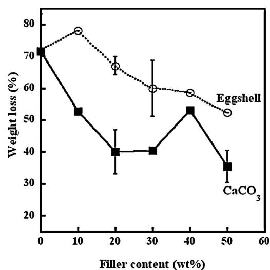
Fig. 5. Weight loss of TPS, TPS/CC composites and TPS/EP composites after the soil burial test for 15 days.
