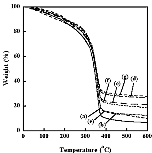
Fig. 7. TGA curves of TPS (a), TPS/CC composites with: 10 wt.% (b), 30 wt.% (c) and 50 wt.% (d) of commercial calcium carbonate and TPS/EP composites with: 10 wt.% (e), 30 wt.% (f) and 50 wt.% (g) of eggshell powder.
