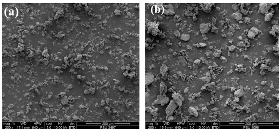
Fig. 1. SEM micrographs of the commercial calcium carbonate (a) and eggshell powder (b).
